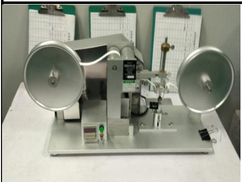
RCA Tape wear-resistant instrument
